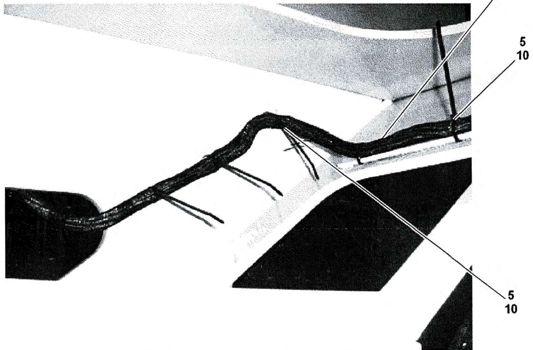
INSIDE RIGHT TURNTABLE HARNESS ROUTING
